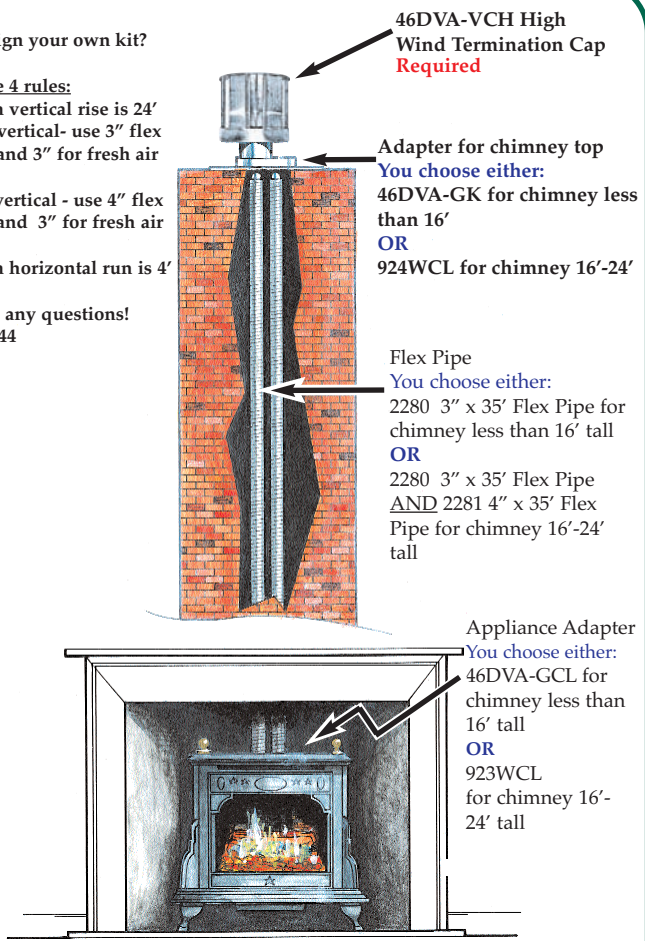
Installation 4 "Into an Existing Fireplace"
