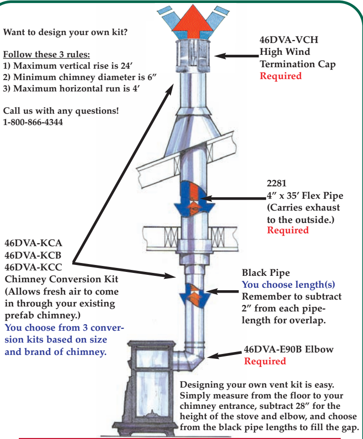
Installation 6 "Into Prefab Chimney up to 24' Tall"
